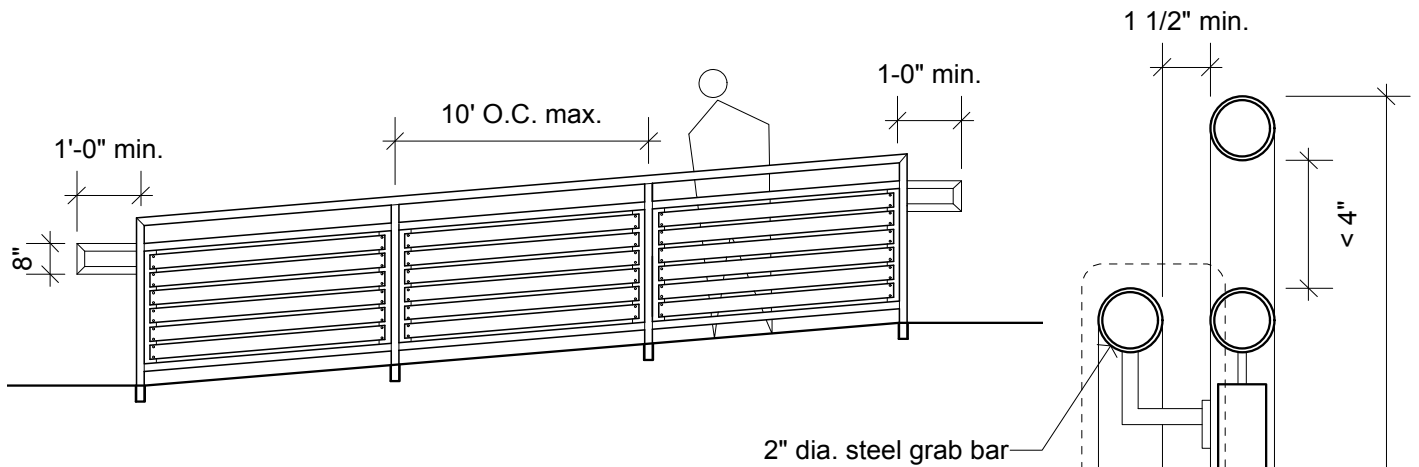
ADA Ramp Guard/Railing Elevation Scale: 1/4" = 1'-0"
