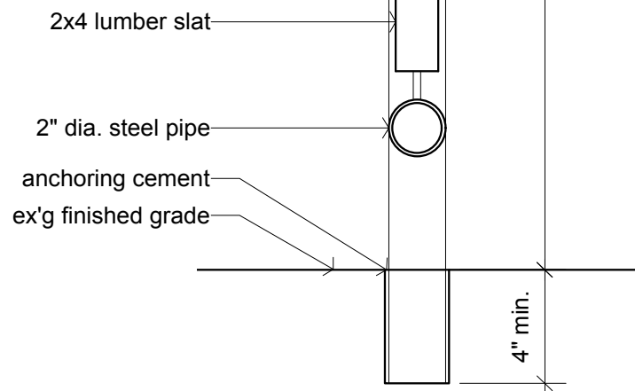
Railing Cross-section Scale: 2" = 1'-0"
