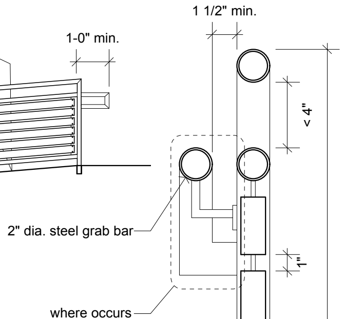
1 ADA Ramp Guard/Railing Elevation Scale: 1/4" = 1'-0"
