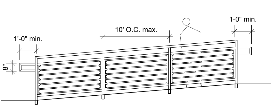
1 ADA Ramp Guard/Railing Elevation Scale: 1/4" = 1'-0"
