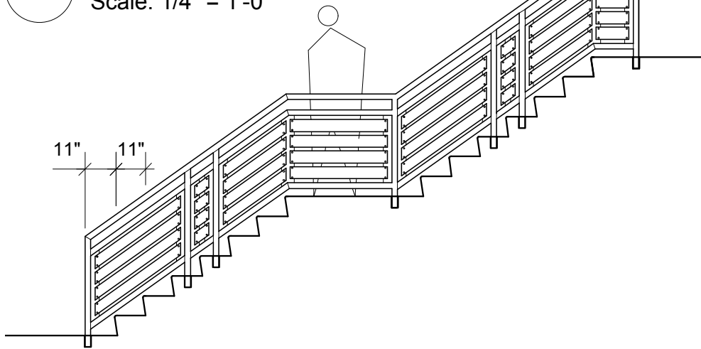
2 Stair Railing Elevation Scale: 1/4" = 1'-0"
