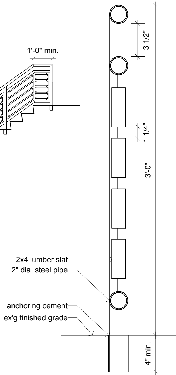
4 Railing Cross-section Scale: 2" = 1'-0"
