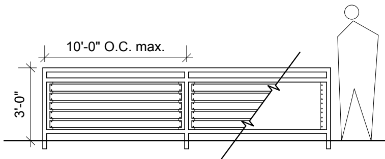
2 Railing Elevation Scale: 1/4" = 1'-0"
