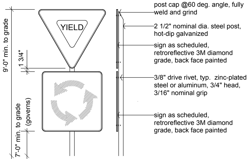
1 Post and Panel Signs Scale: 1/2" = 1'-0"
