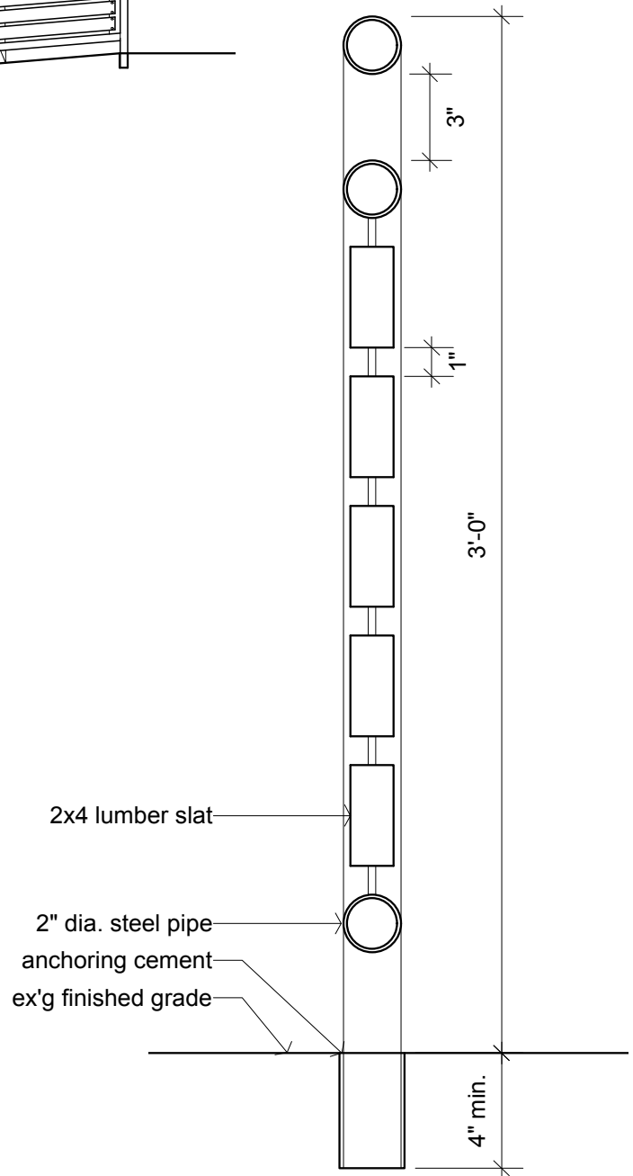
4 Railing Cross-section Scale: 2" = 1'-0"
