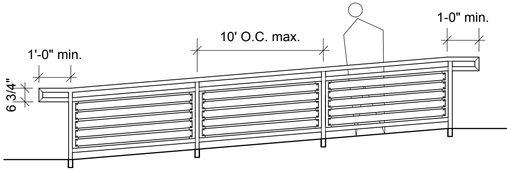
1 ADA Ramp Railing Elevation Scale: 1/4" = 1'-0"
