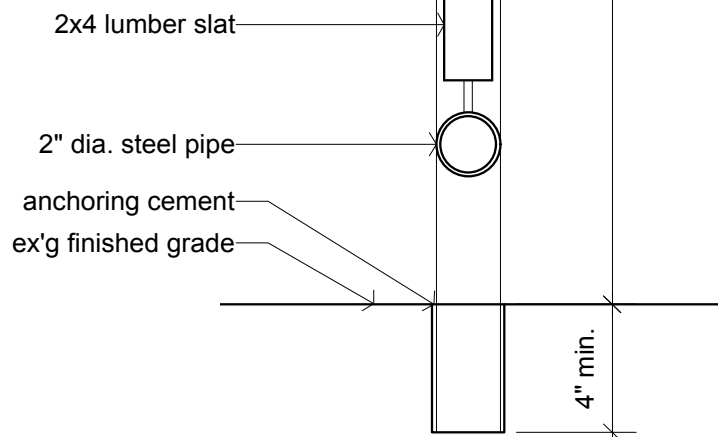
4 Railing Cross-section Scale: 2" = 1'-0"
