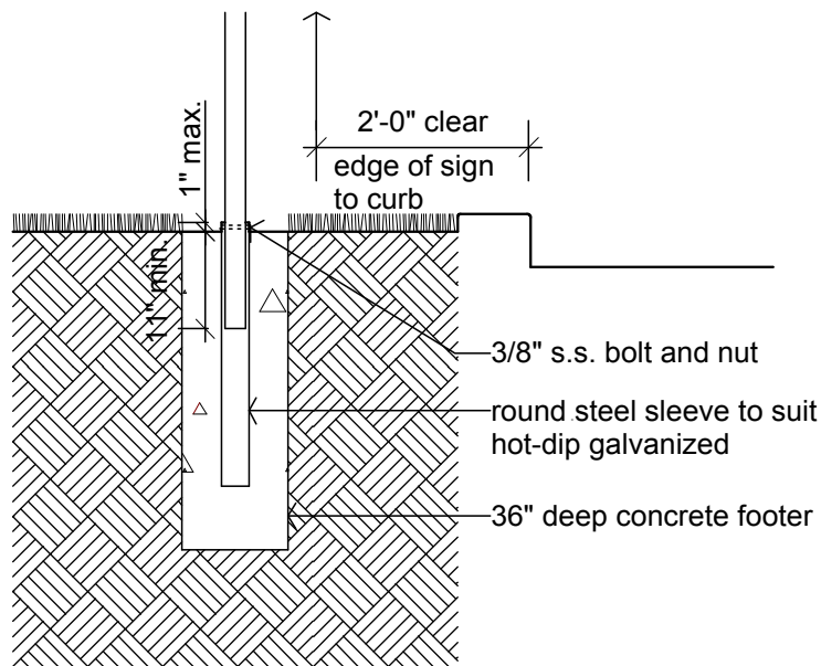
2 Post and Panel Sign Base Scale: 1/2" = 1'-0"
