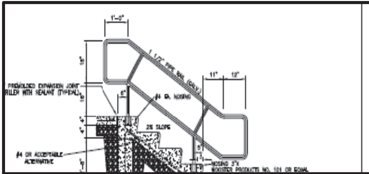
Railing Detail
