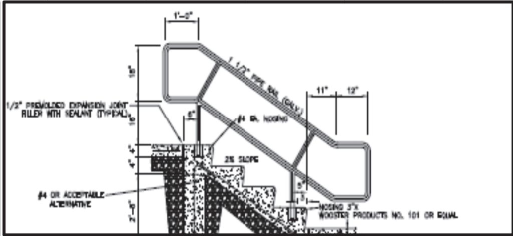
Hand-rail Detail
