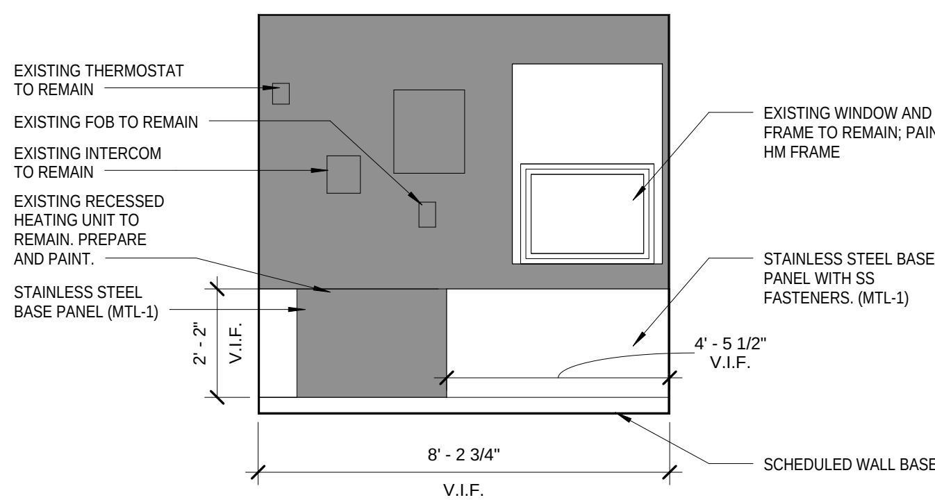
5 INTERIOR ELEVATION 3/8" = 1'-0"
