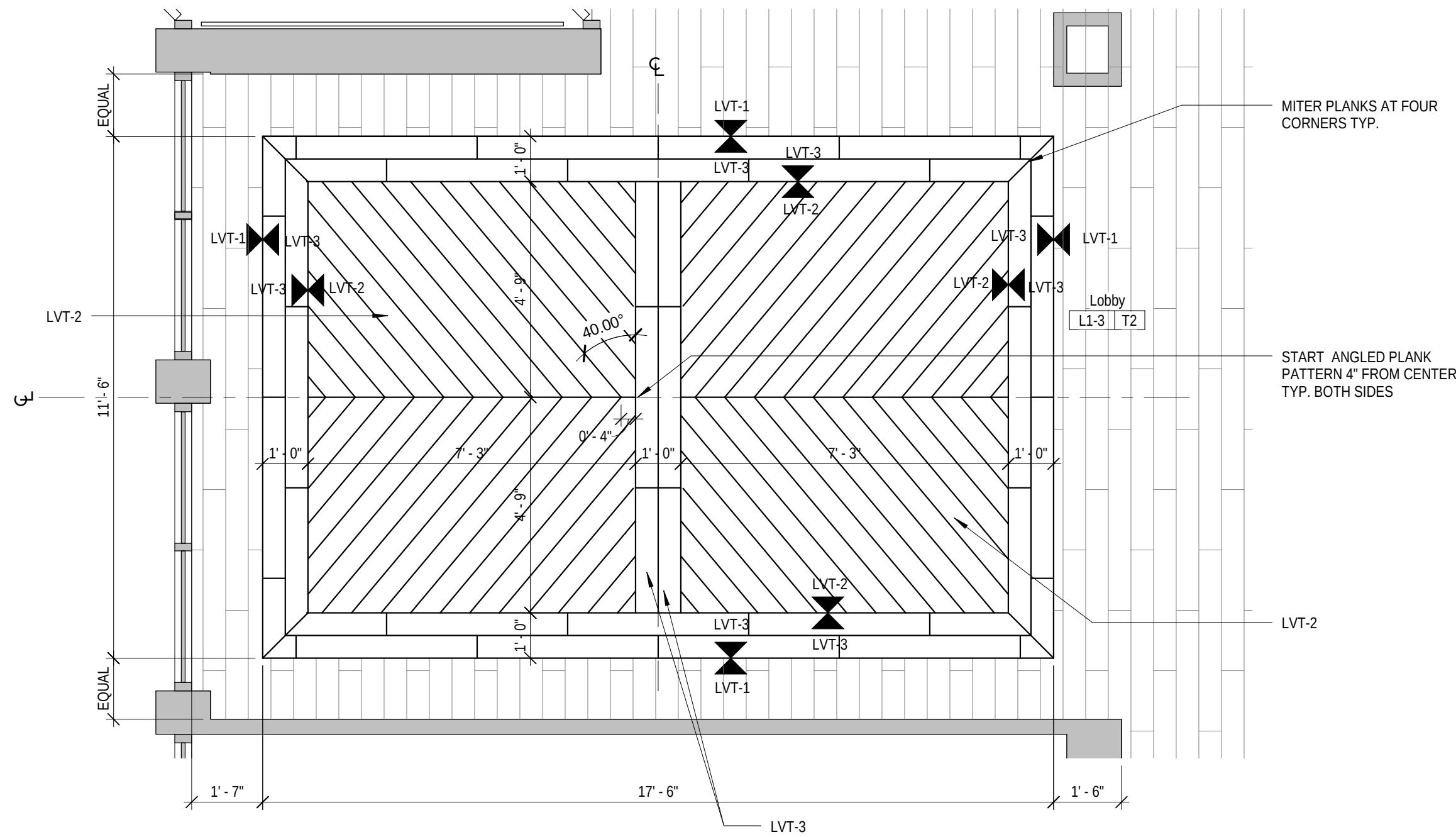
3 FIRST FLOOR FINISH PLAN - FLOOR PATTERN DETAIL 3/8" = 1'-0"
