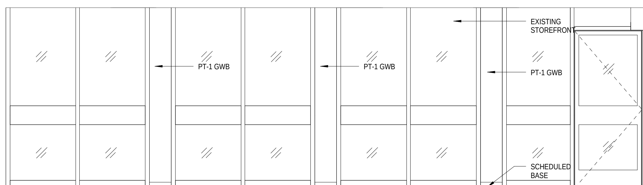
12 INTERIOR ELEVATION 3/8" = 1'-0"
