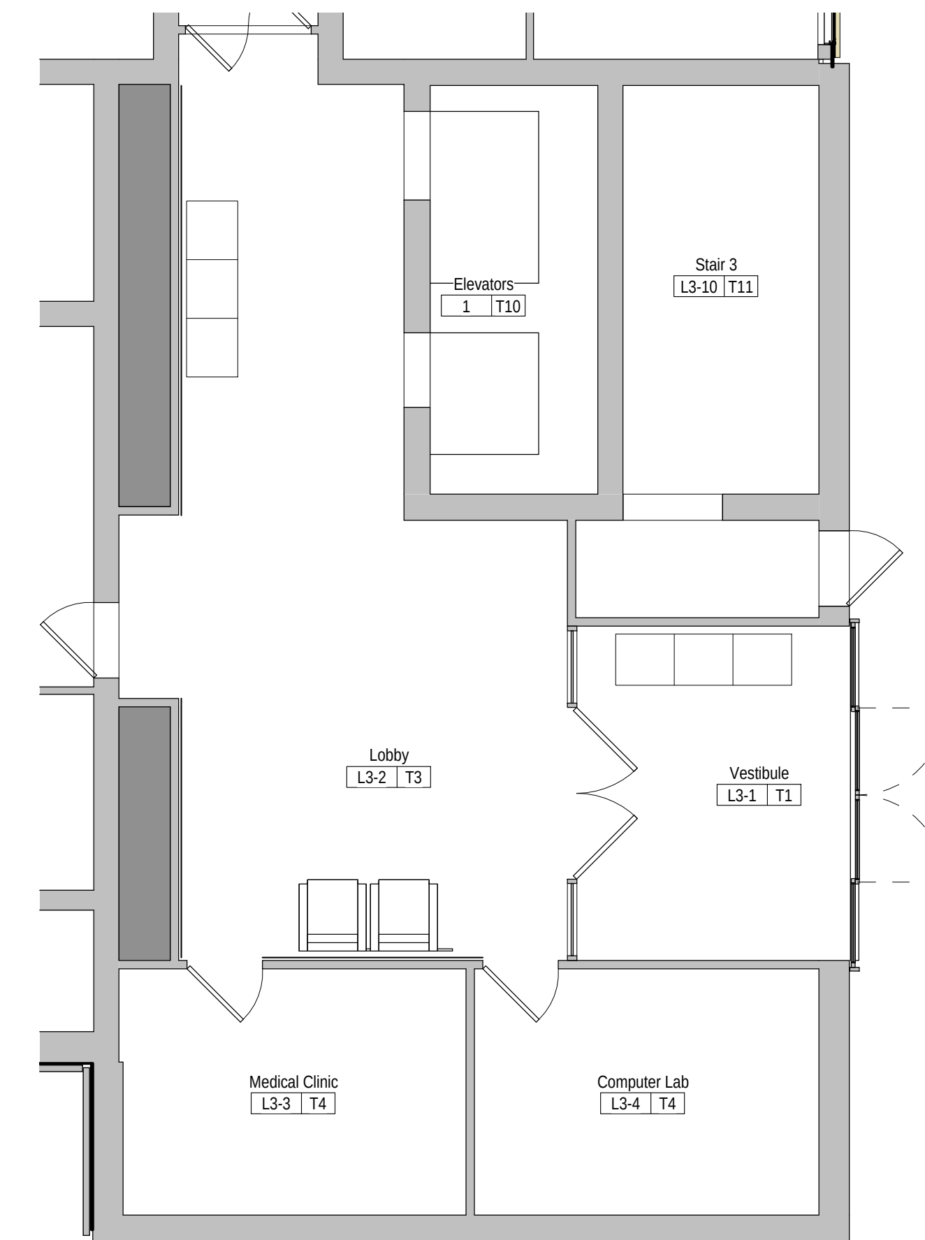
2 THIRD FLOOR REFERENCE FURNITURE PLAN 3/16" = 1'-0"
