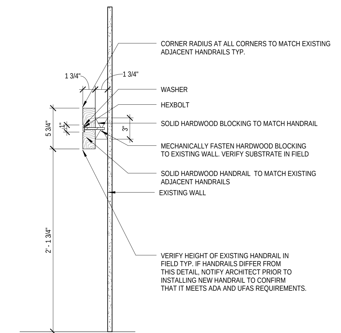
9 SECTION- HANDRAIL TYPICAL 1 1/2" = 1'-0"
