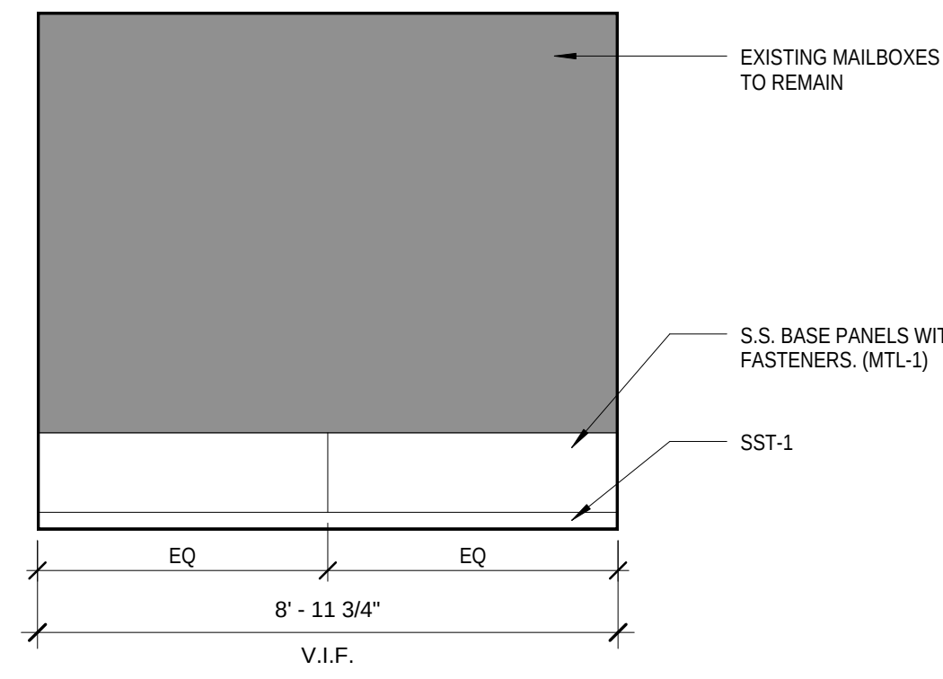
1 INTERIOR ELEVATION 3/8" = 1'-0"
