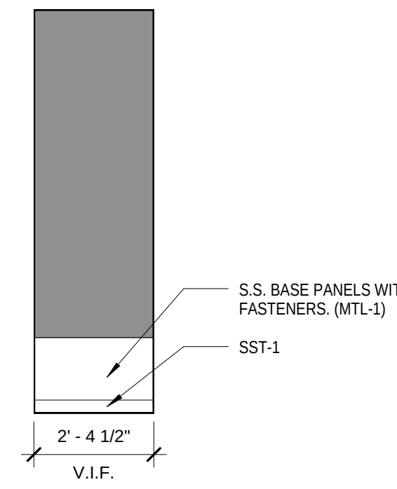
2 INTERIOR ELEVATION 3/8" = 1'-0"
