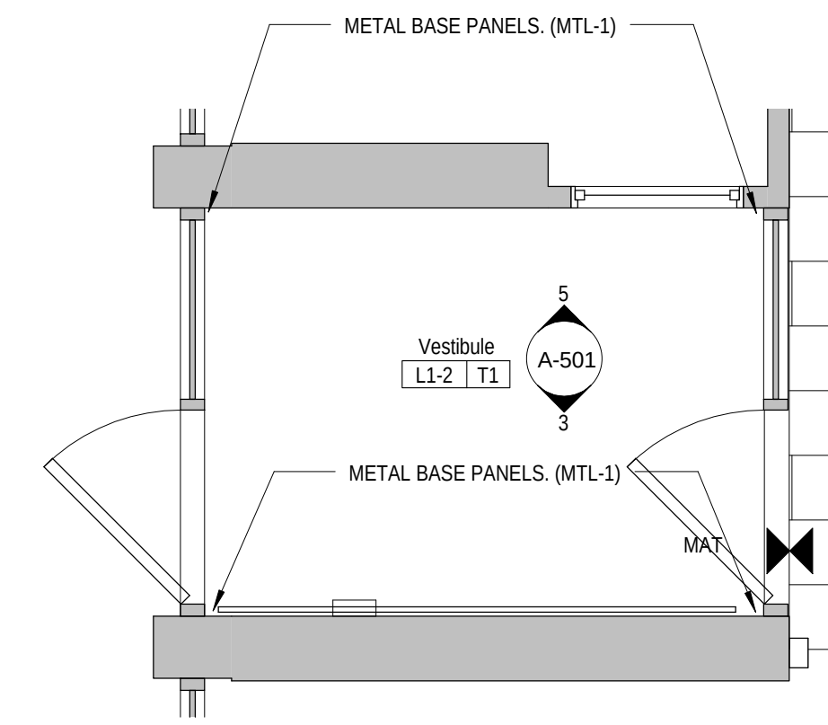
6 ENLARGED FLOOR PLAN 3/8" = 1'-0"
