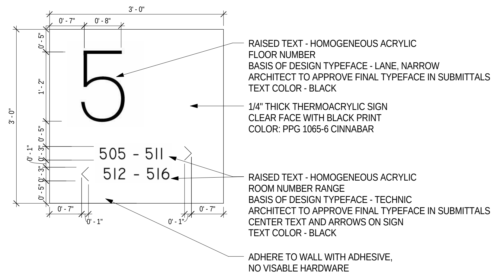
11 DIRECTIONAL SIGN DETAIL 1" = 1'-0"
