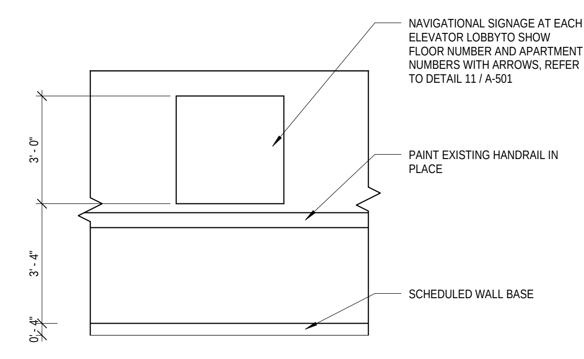
7 INTERIOR ELEVATION 3/8" = 1'-0"
