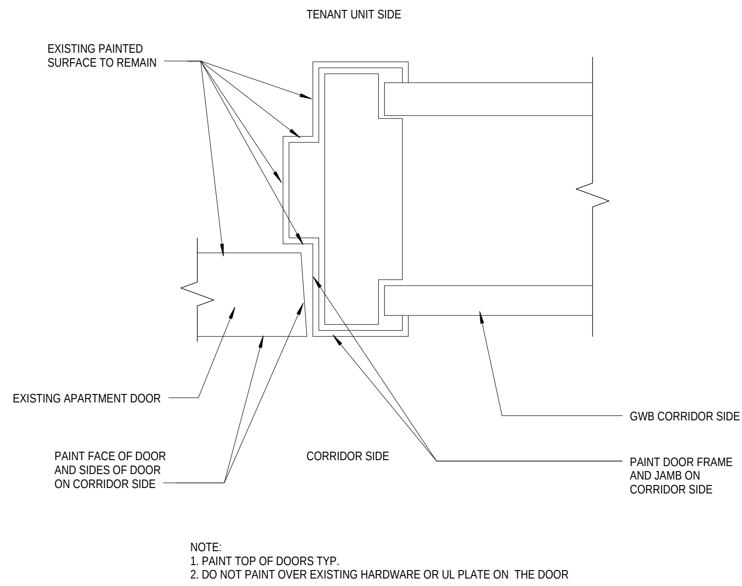
5 TYPICAL DOOR FRAME PAINT DETAIL 6" = 1'-0"
