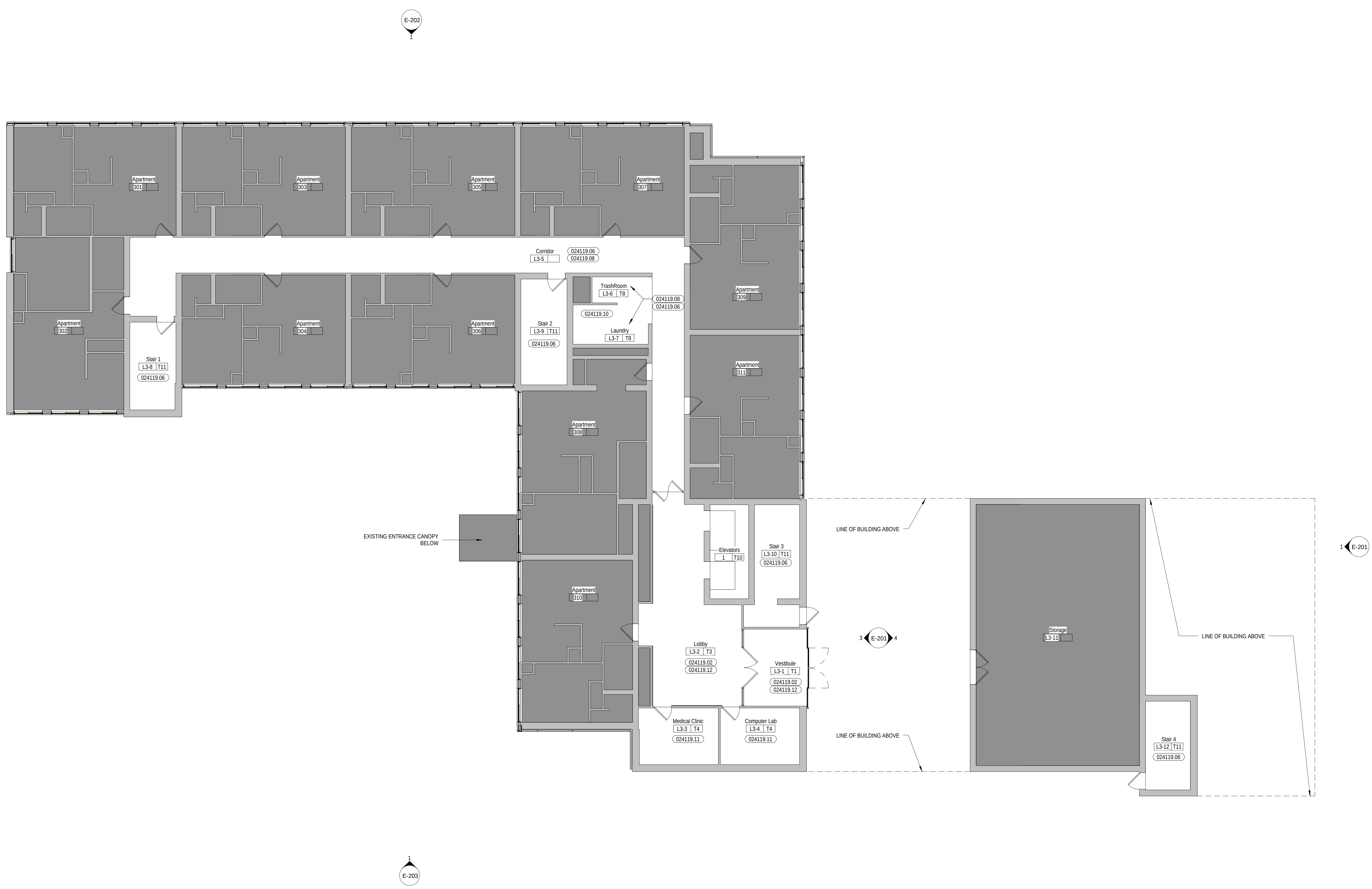
1 THIRD FLOOR DEMOLITION PLAN 1/8" = 1'-0"
