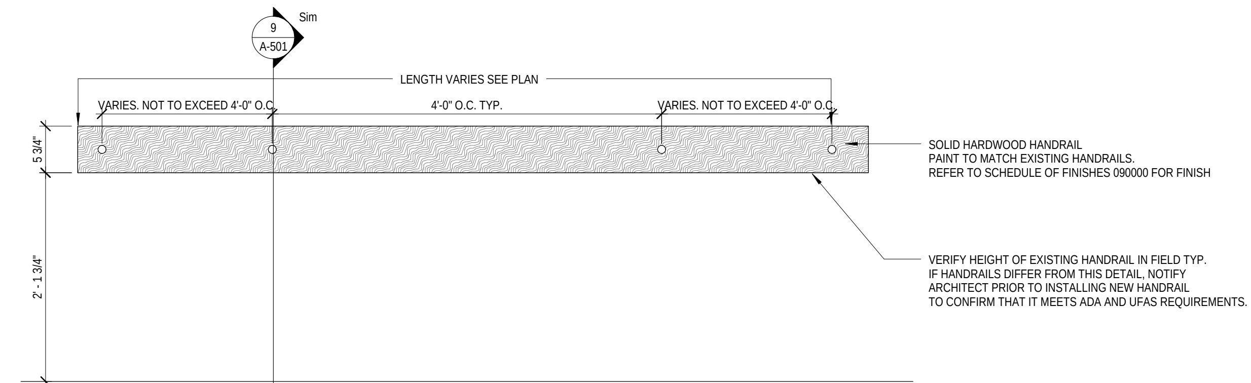
4 ELEVATION- HANDRAIL TYPICAL 1" = 1'-0"
