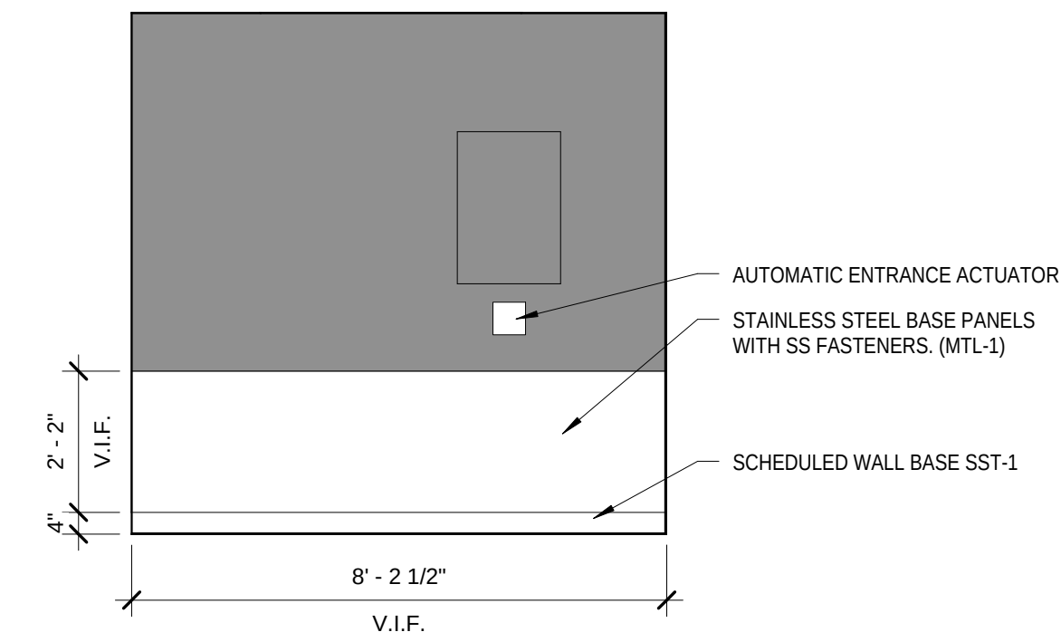
3 INTERIOR ELEVATION 3/8" = 1'-0"
