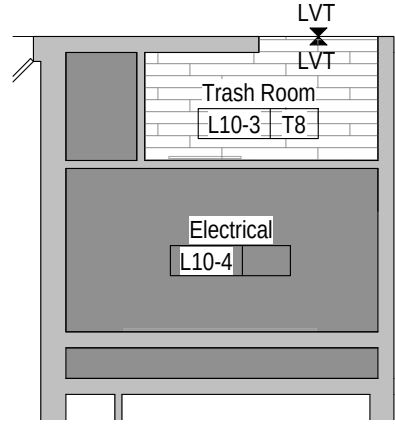
2 TENTH FLOOR TRASH ROOM PLAN 1/8" = 1'-0" ELEVATION 1213' - 6"
