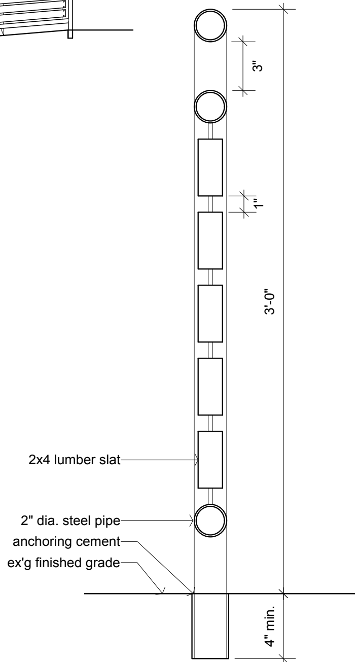
4 Railing Cross-section Scale: 2" = 1'-0"
